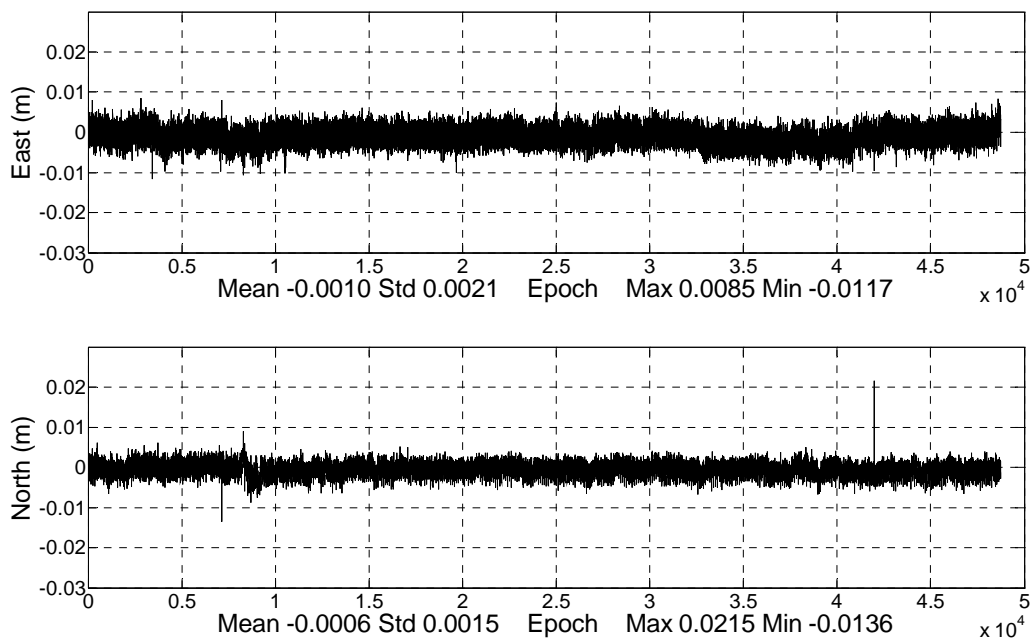
Figure 6 East and North error for long term (13.5 hour) static positioning test.
