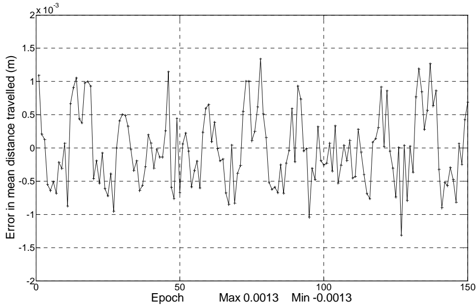
Figure 11 Error in 1cm moves from mean static positions (simulated deformation movement test).
