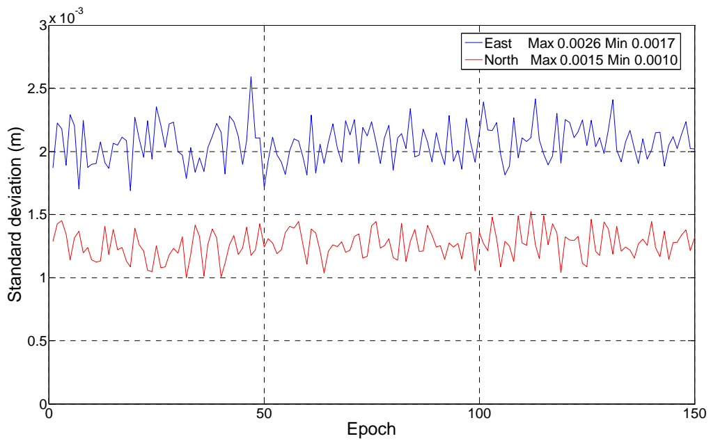
Figure 10 Standard deviation of static East North positions (simulated deformation movement test).
