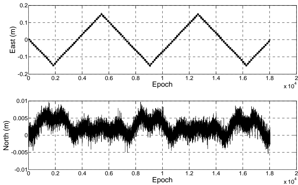
Figure 8 East North time series (simulated deformation movement test).
