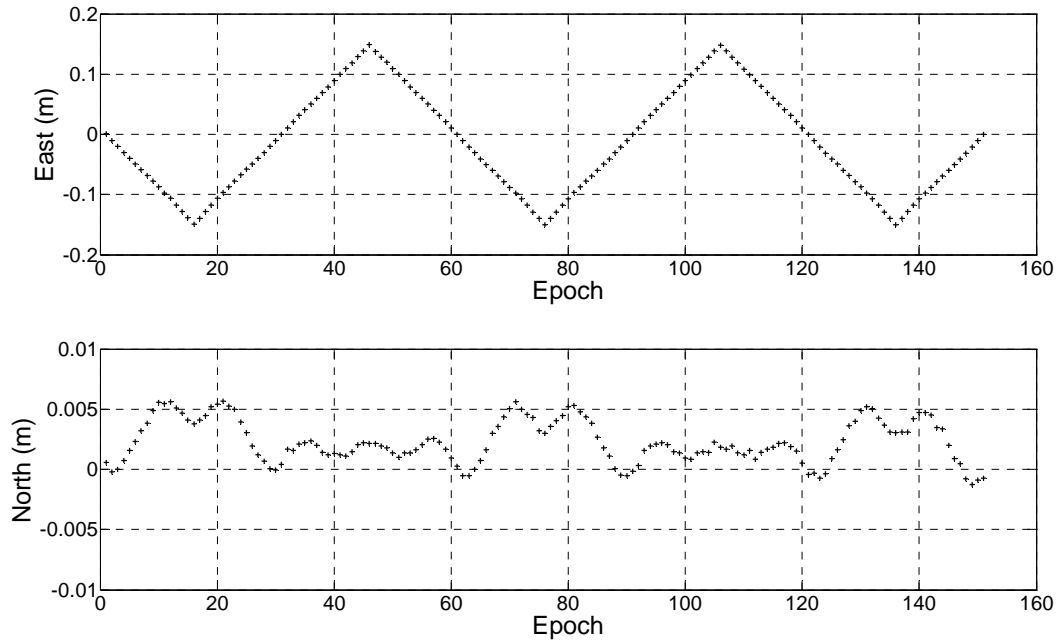
Figure 9 Mean static East North positions (simulated deformation movement test).
