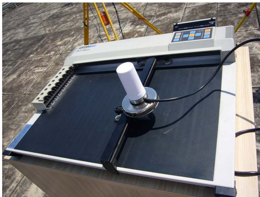
Figure 4 Locata receiver antenna setup using Roland DXY-980A plotter table.
