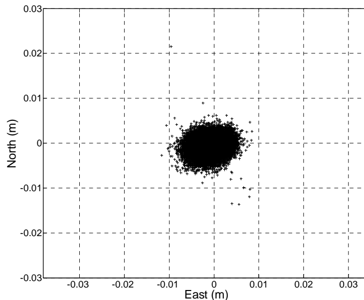
Figure 5 Horizontal error scatter plot for long term (13.5 hour) static positioning test.
