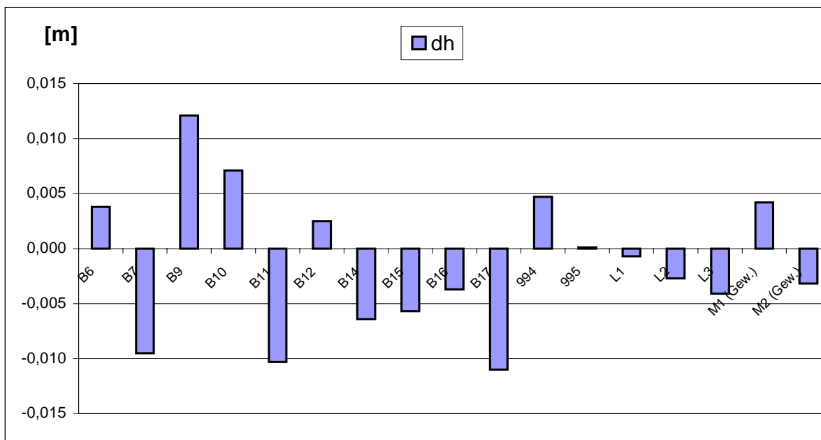
Fig. 9: Differences between the heights of the RTK-solution using the reference station Karlsruhe and the levelling heights
