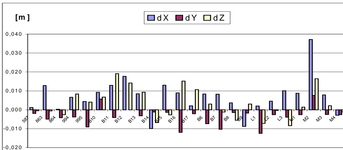
Fig. 4: Differences (dX, dY, dZ) between two 10sec measurements of the local RTK-version
