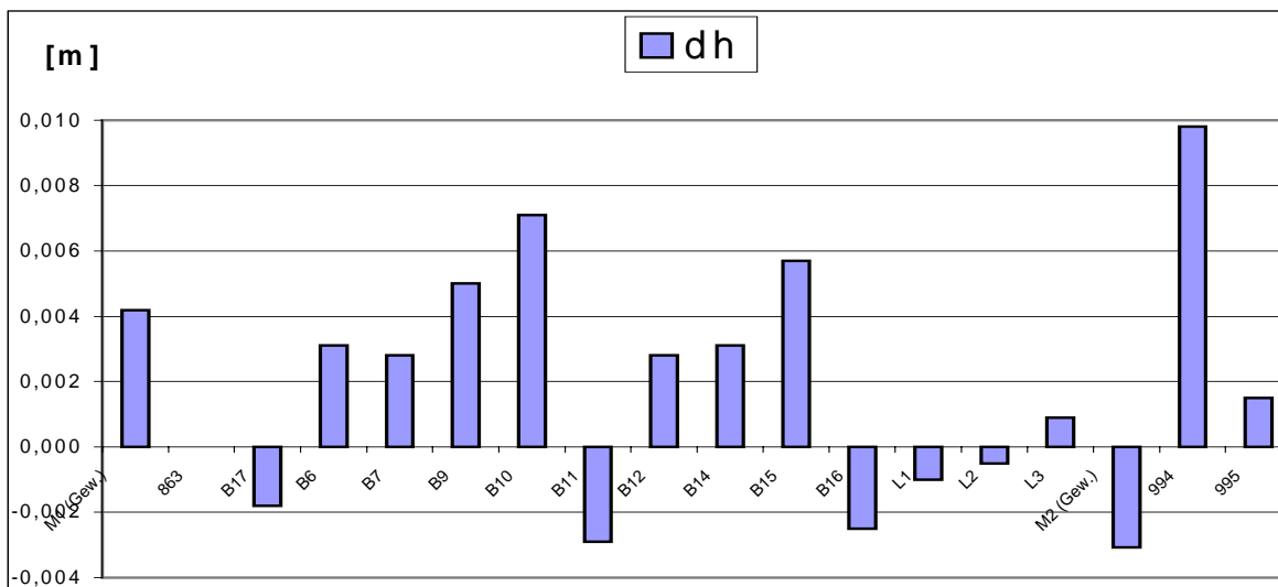
Fig. 7: Differences between the heights of the local RTK-version and the levelling heights
