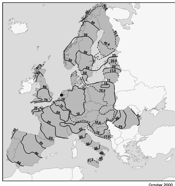
Figure 4: UELN 95/98 – Isoline of Precision [kgal . mm]
